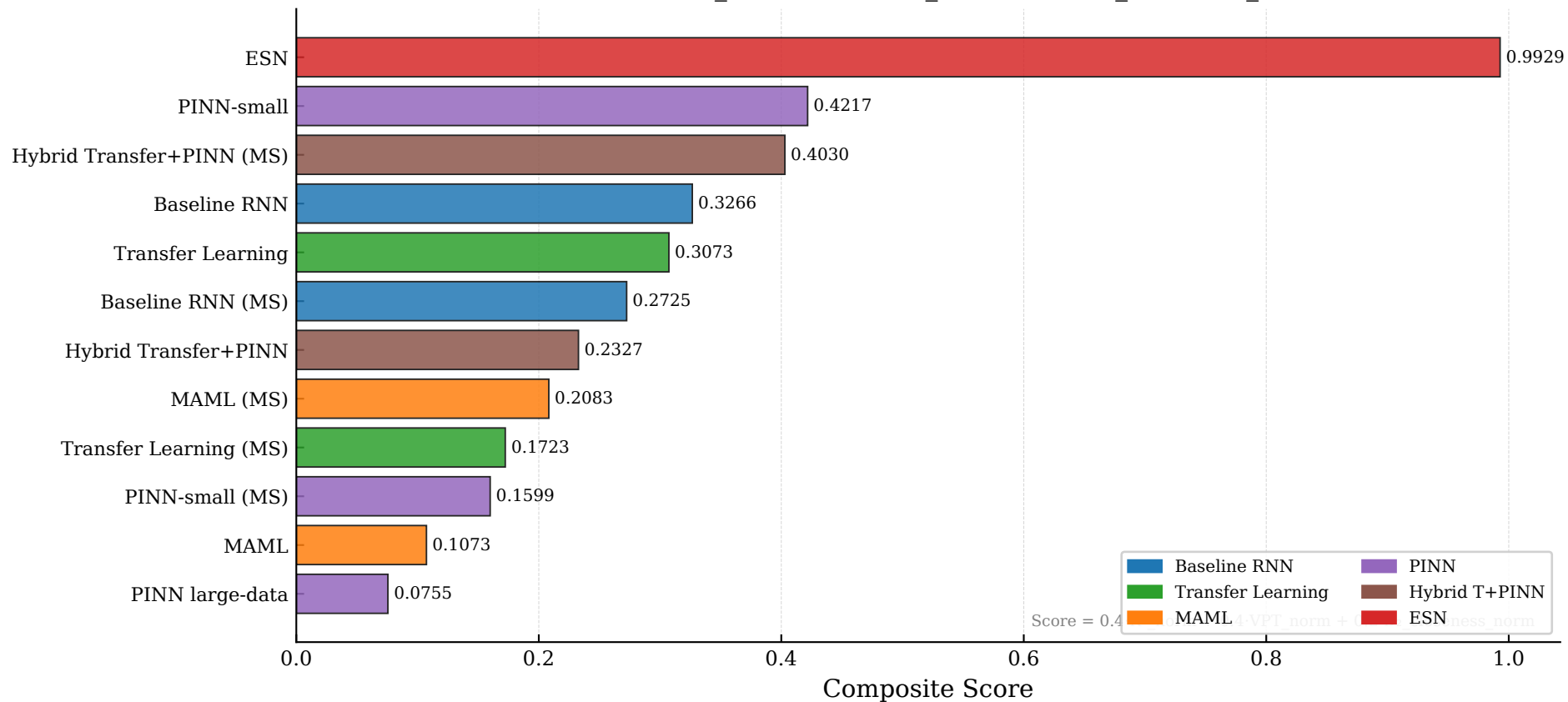
Duffing — Three-Metric Composite Leaderboard Score = 0.4 \cdot R^2_{\text{norm}} + 0.4 \cdot \text{VPT}_{\text{norm}} + 0.2 \cdot D_2_{\text{closeness}_{\text{norm}}}
